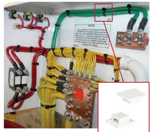
Wire Mounting
